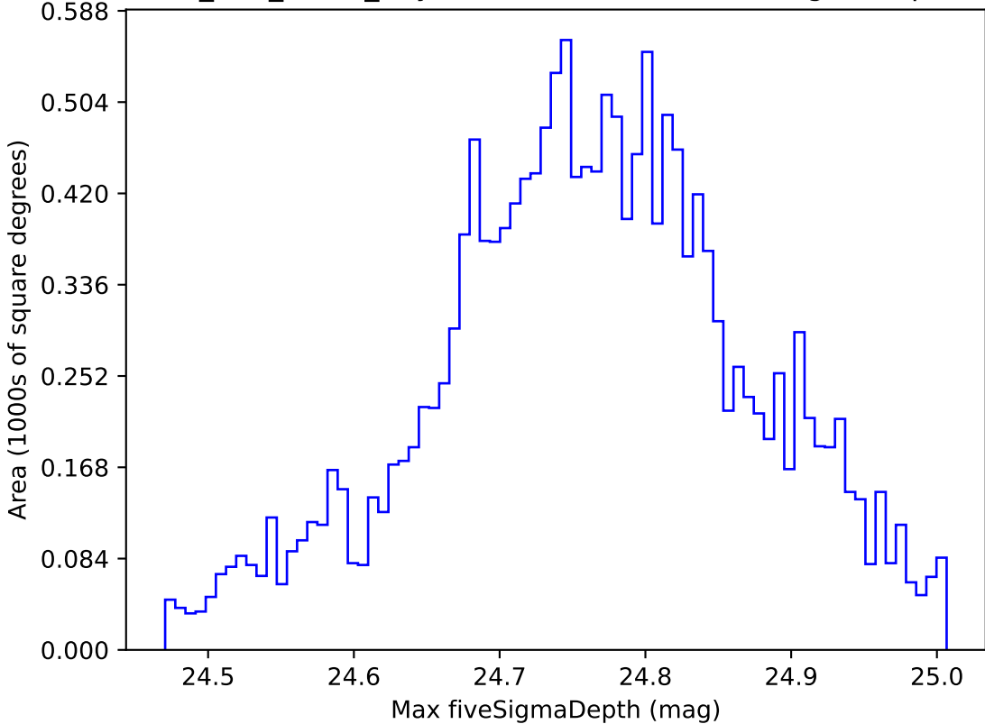
too_100_1v3.4_10yrs WFD r band: Max fiveSigmaDepth
