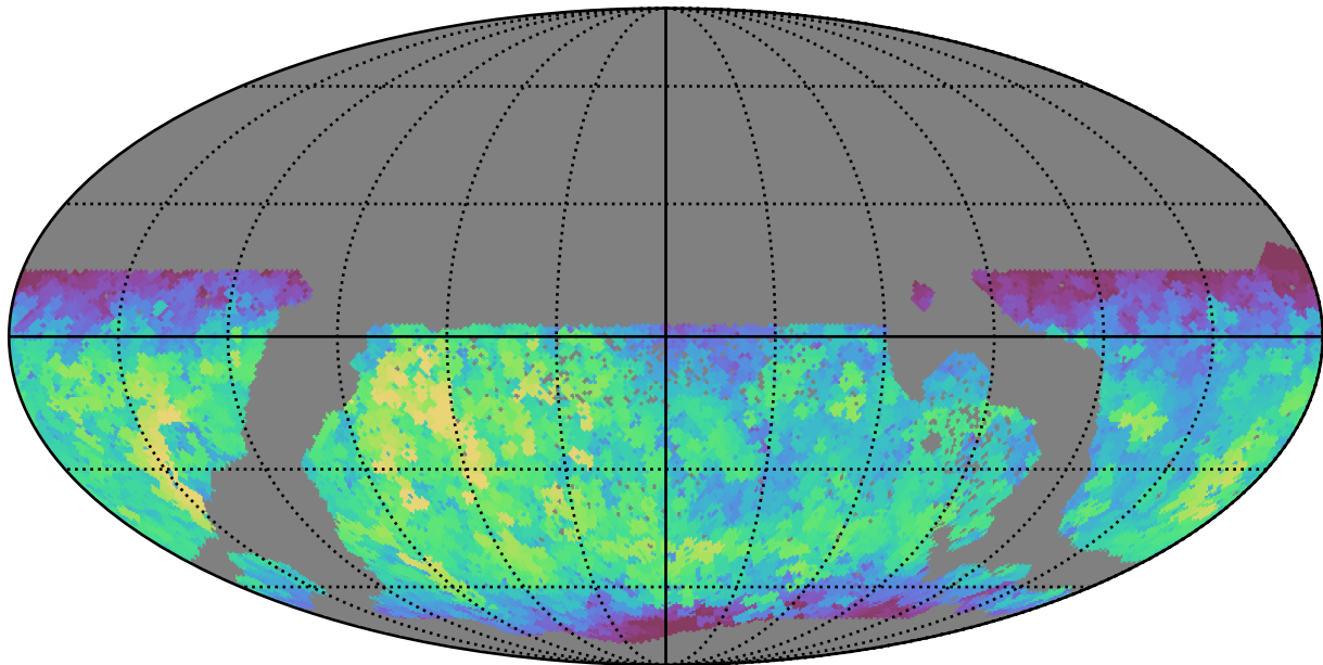
too_100_1v3.4_10yrs WFD i band: Max fiveSigmaDepth
