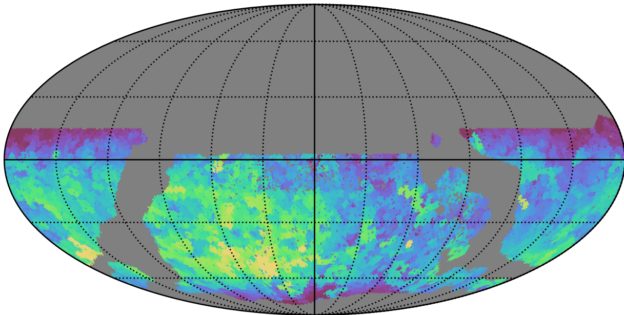
too_100_1v3.4_10yrs WFD g band: Max fiveSigmaDepth
