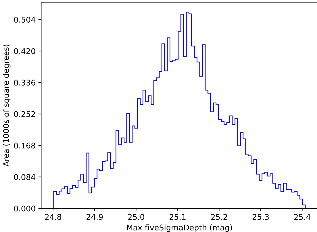
too_100_1v3.4_10yrs WFD g band: Max fiveSigmaDepth
