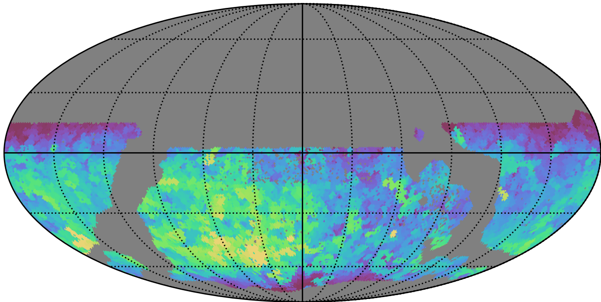
too_100_1v3.4_10yrs WFD all bands: Max fiveSigmaDepth
