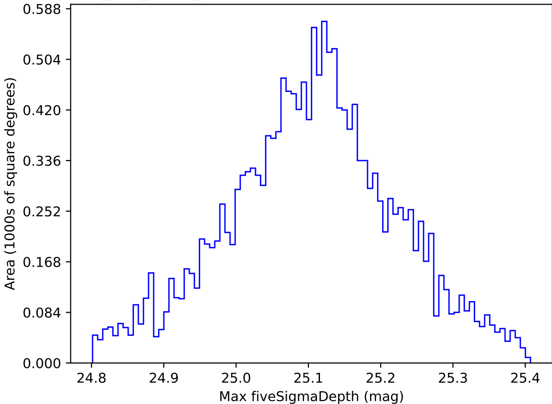
too_100_1v3.4_10yrs WFD all bands: Max fiveSigmaDepth
