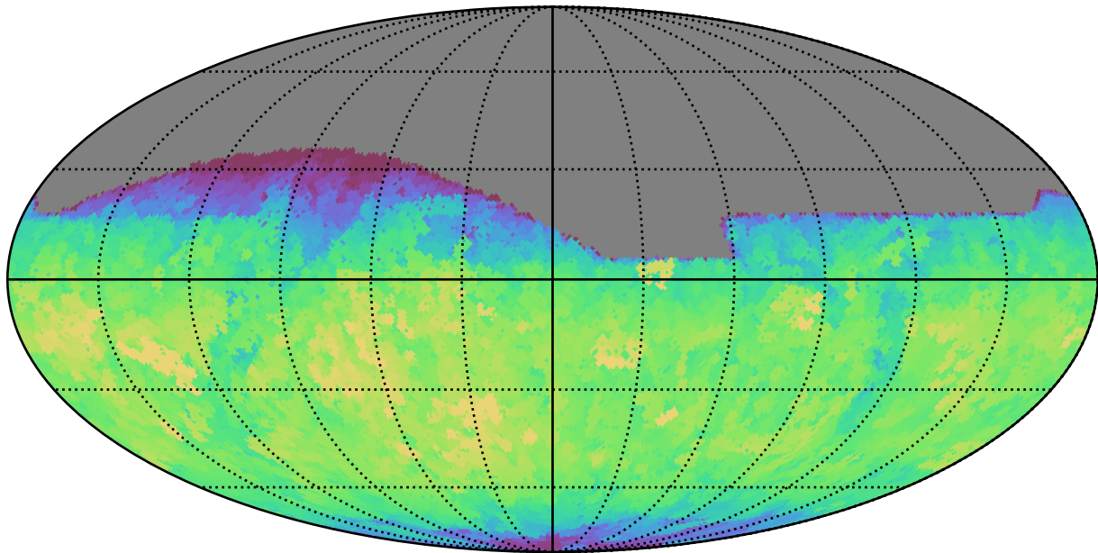
too_100_1v3.4_10yrs All sky z band: Max fiveSigmaDepth
