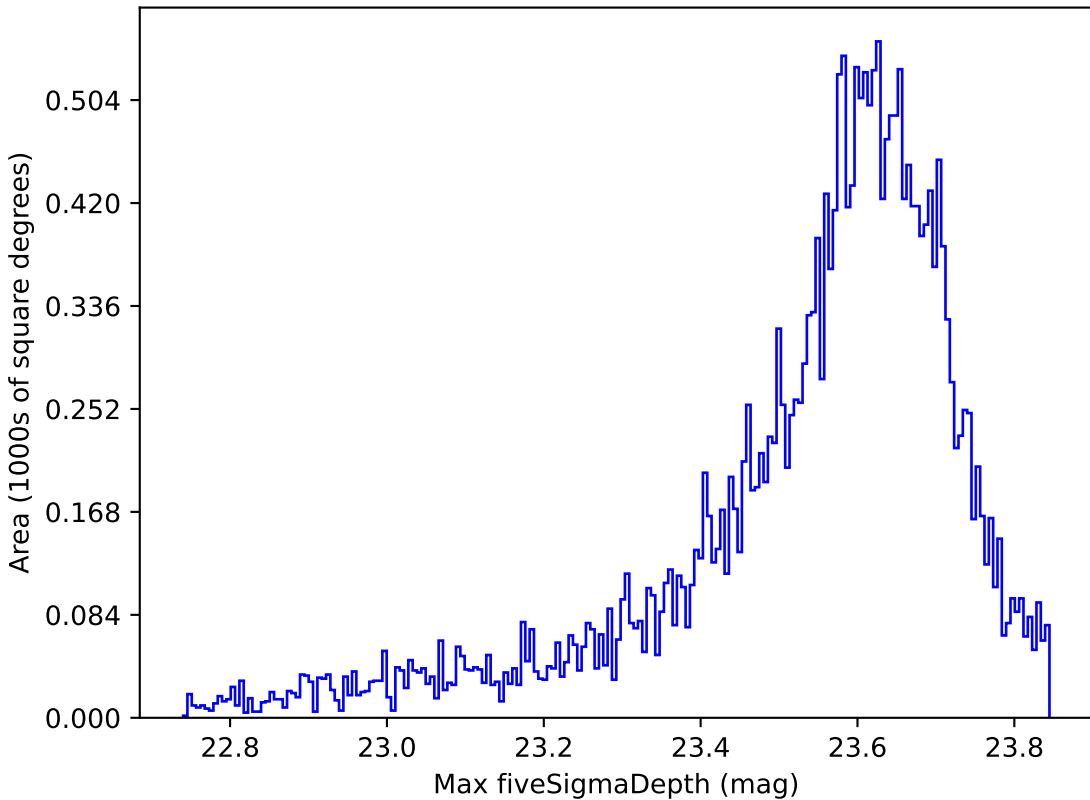
too_100_1v3.4_10yrs All sky z band: Max fiveSigmaDepth
