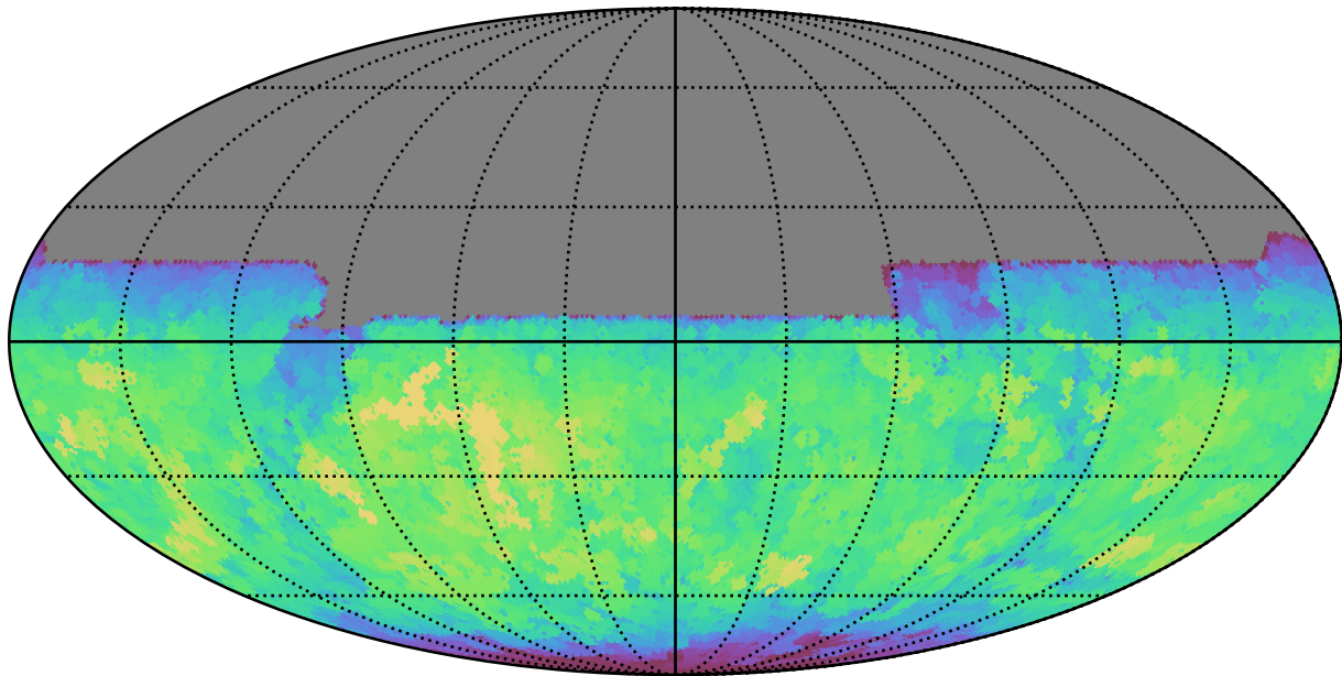
too_100_1v3.4_10yrs All sky y band: Max fiveSigmaDepth
