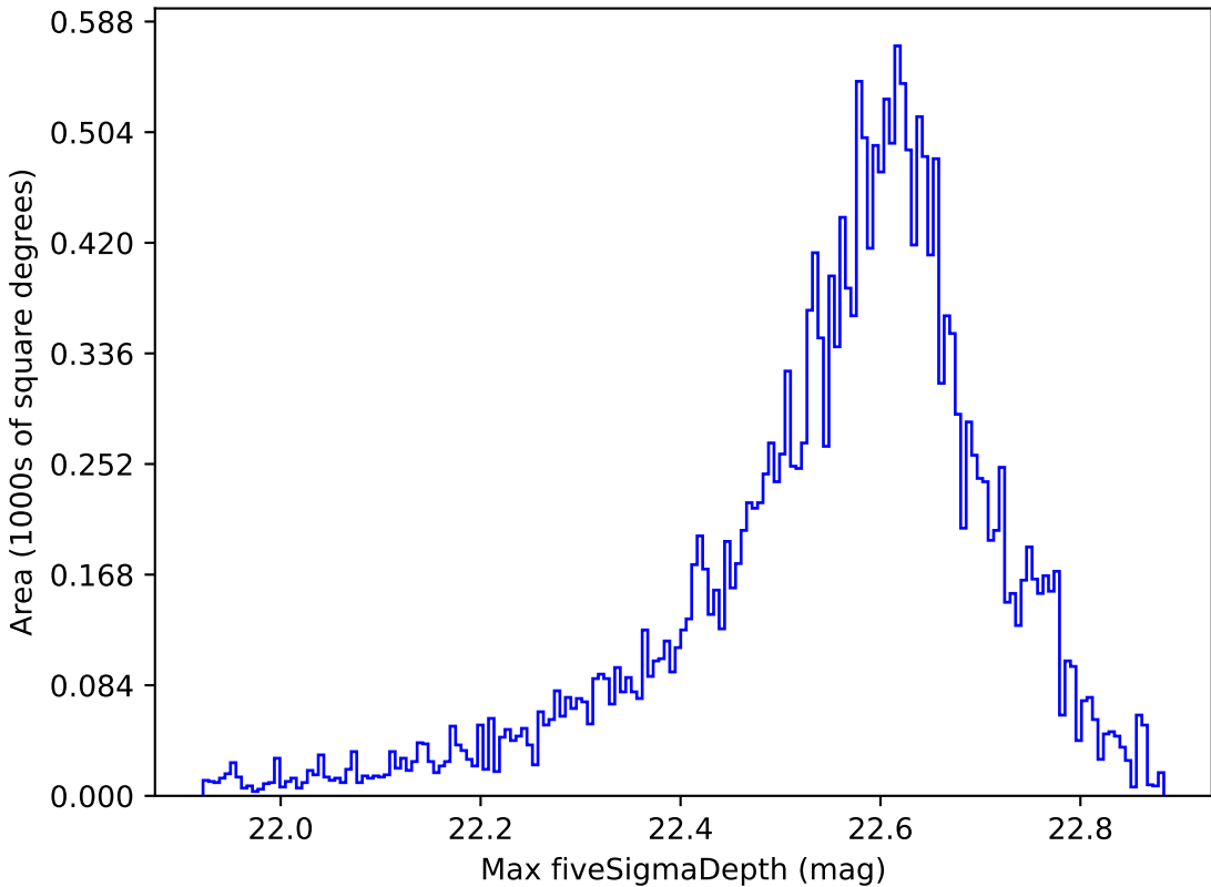
too_100_1v3.4_10yrs All sky y band: Max fiveSigmaDepth
