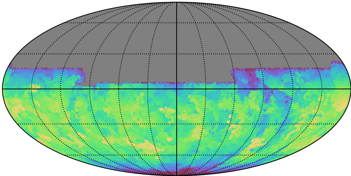
too_100_1v3.4_10yrs All sky u band: Max fiveSigmaDepth
