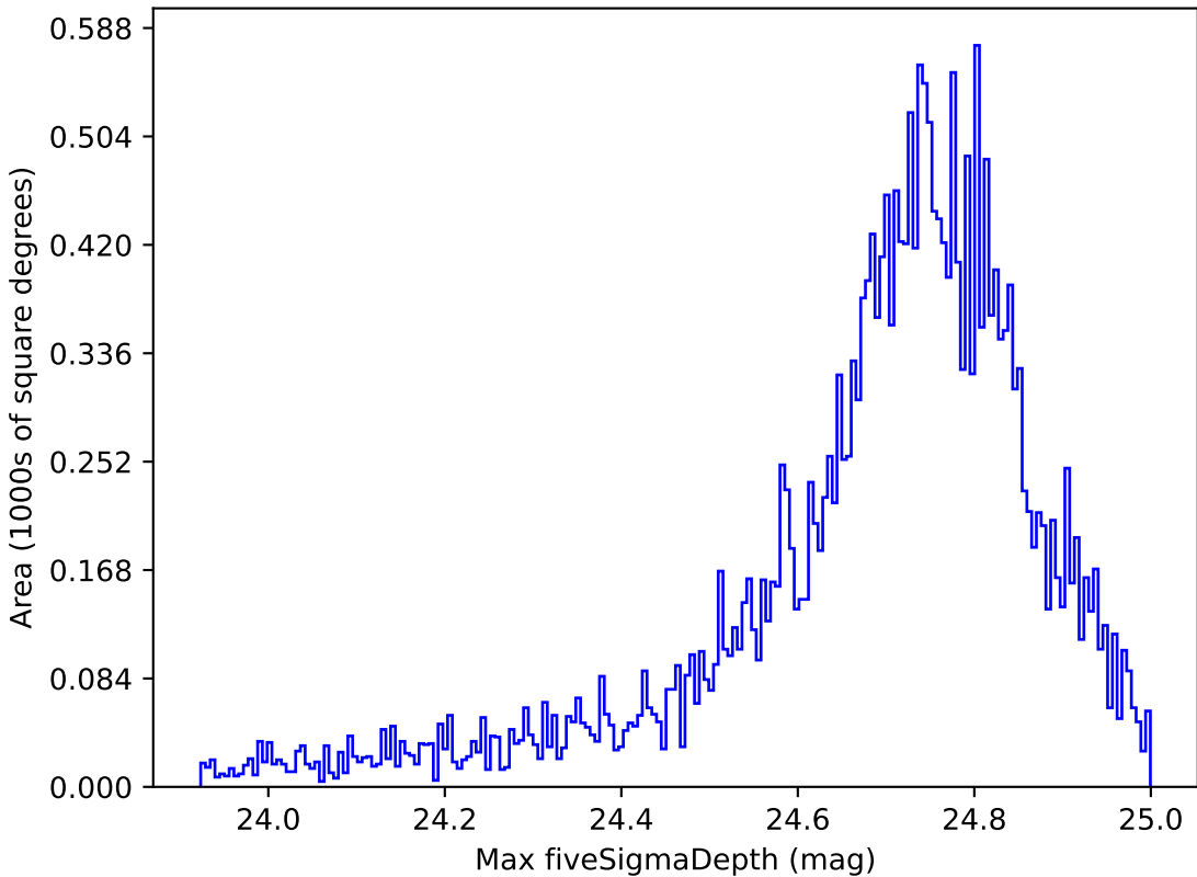
too_100_1v3.4_10yrs All sky r band: Max fiveSigmaDepth
