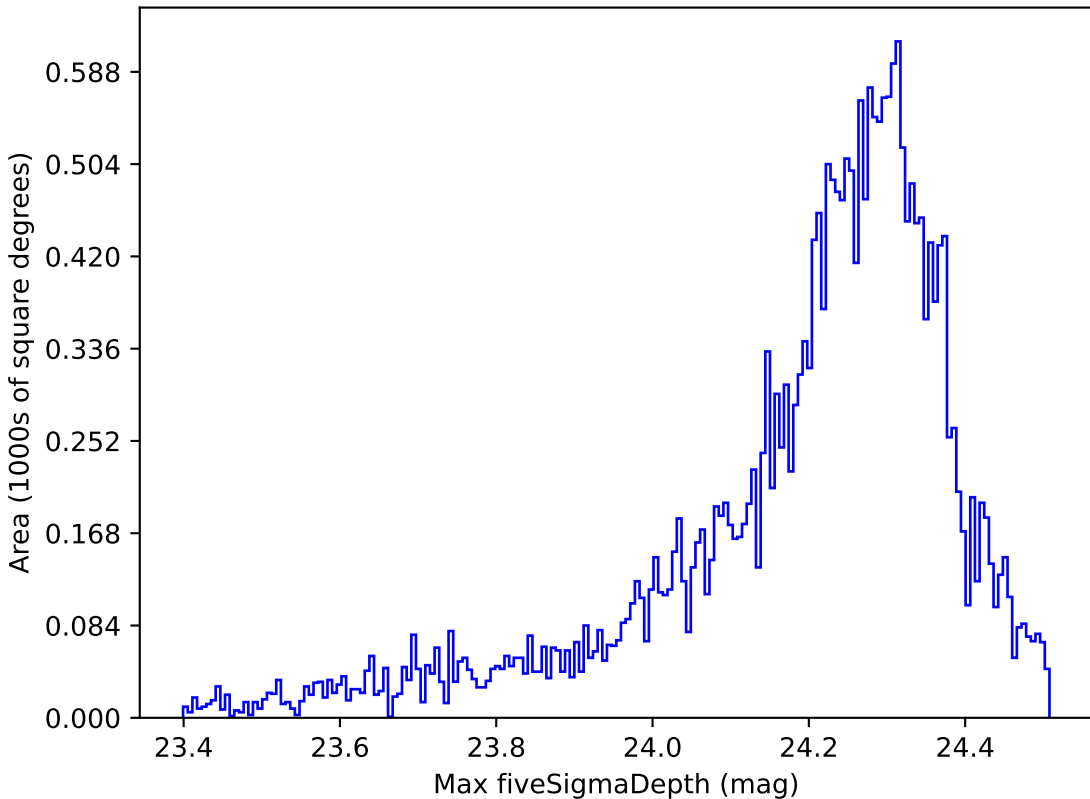
too_100_1v3.4_10yrs All sky i band: Max fiveSigmaDepth
