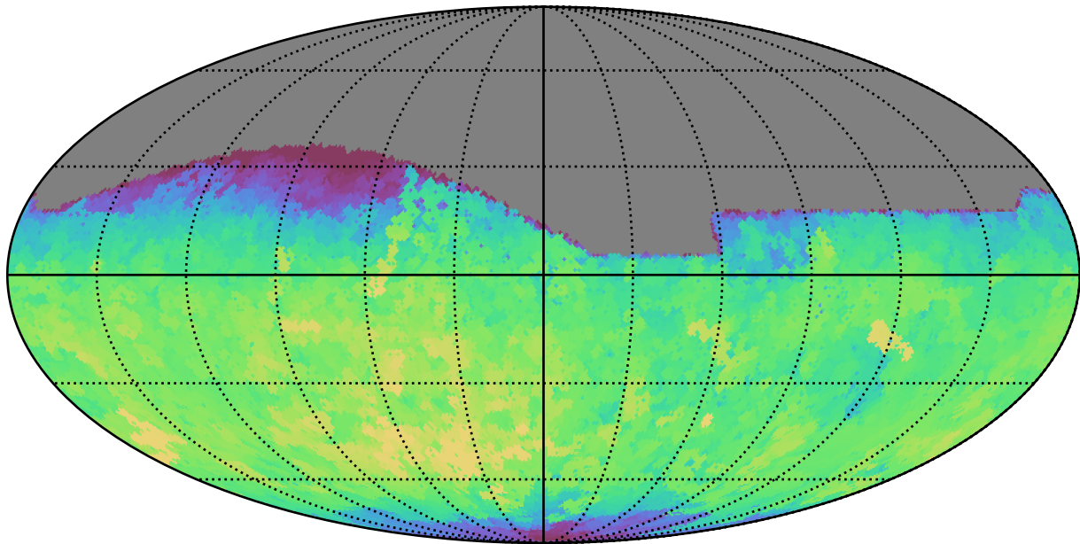
too_100_1v3.4_10yrs All sky g band: Max fiveSigmaDepth
