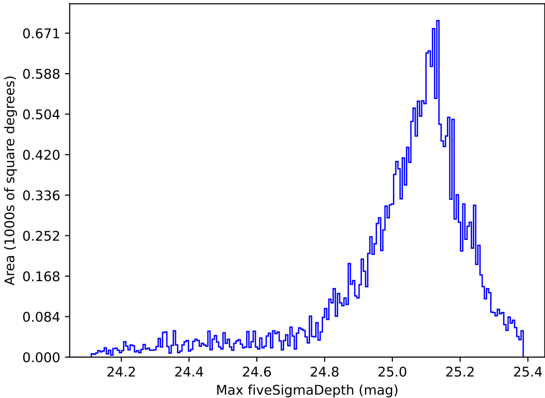
too_100_1v3.4_10yrs All sky all bands: Max fiveSigmaDepth
