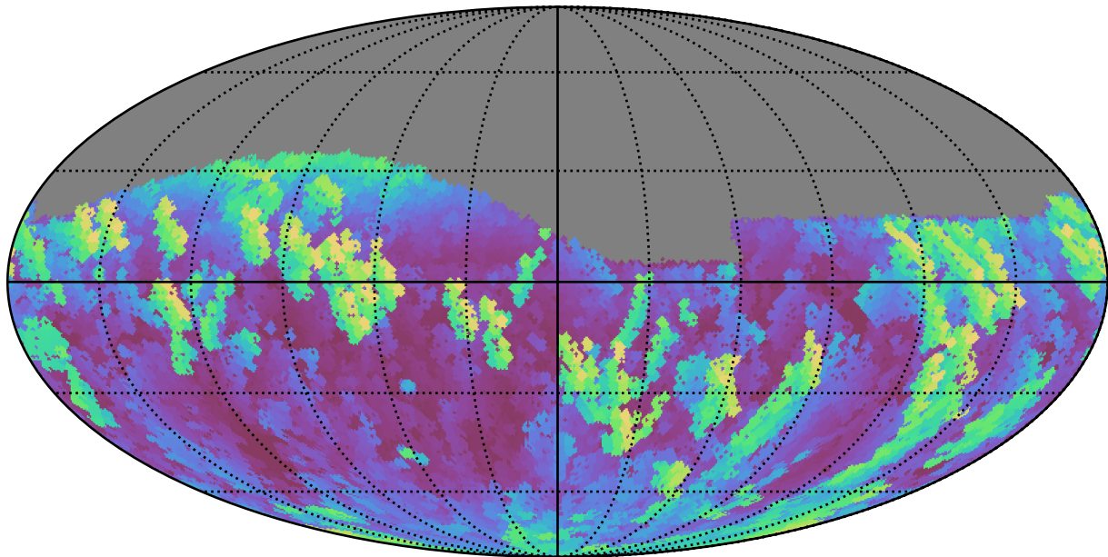
too_100_1v3.4_10yrs Yr 1 z band: Max airmass
