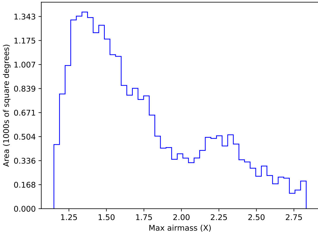
too_100_1v3.4_10yrs Yr 1 z band: Max airmass
