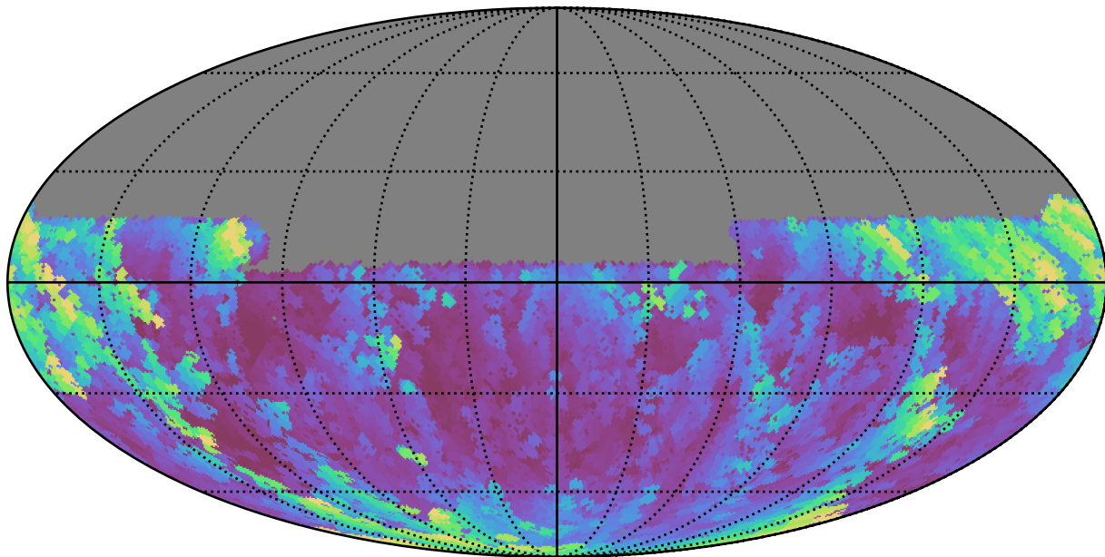
too_100_1v3.4_10yrs Yr 1 y band: Max airmass
