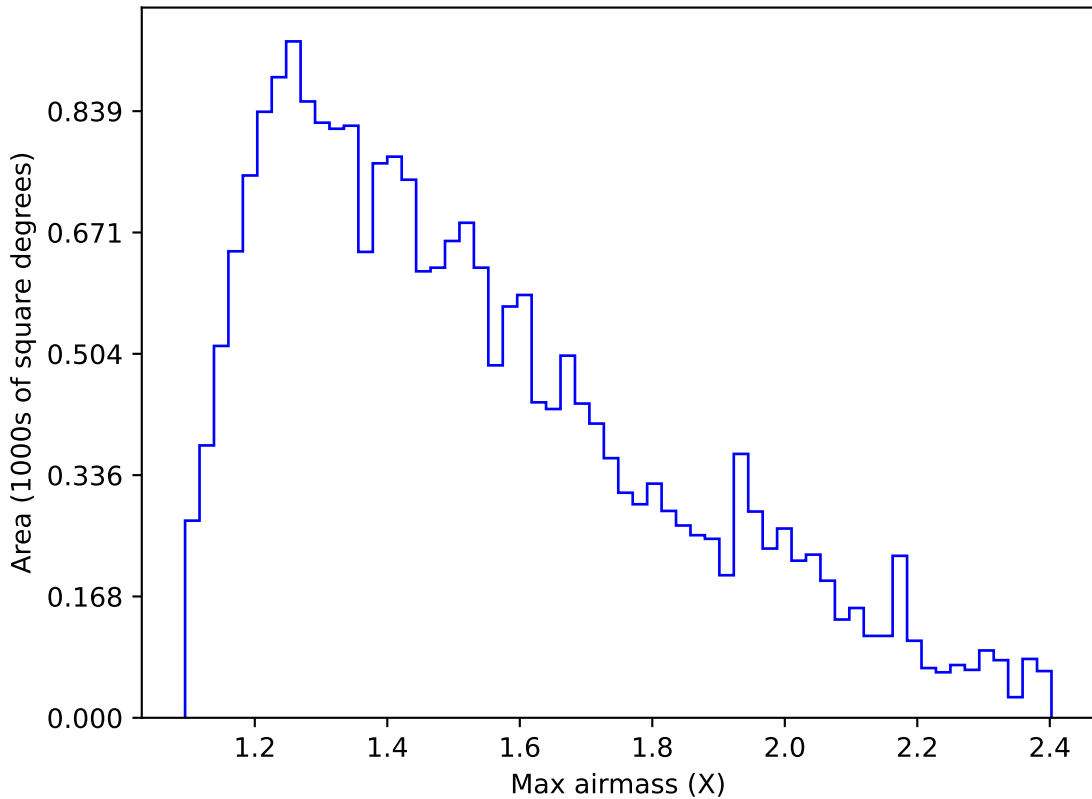
too_100_1v3.4_10yrs Yr 1 u band: Max airmass
