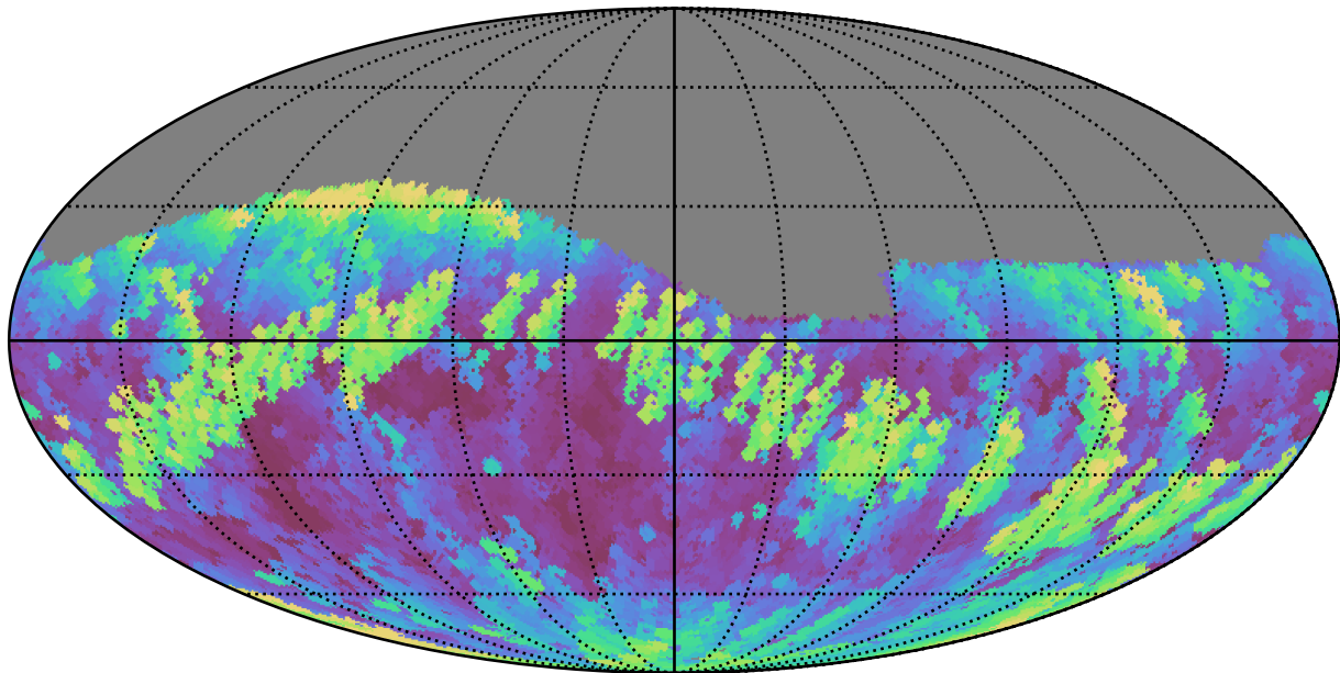
too_100_1v3.4_10yrs Yr 1 r band: Max airmass
