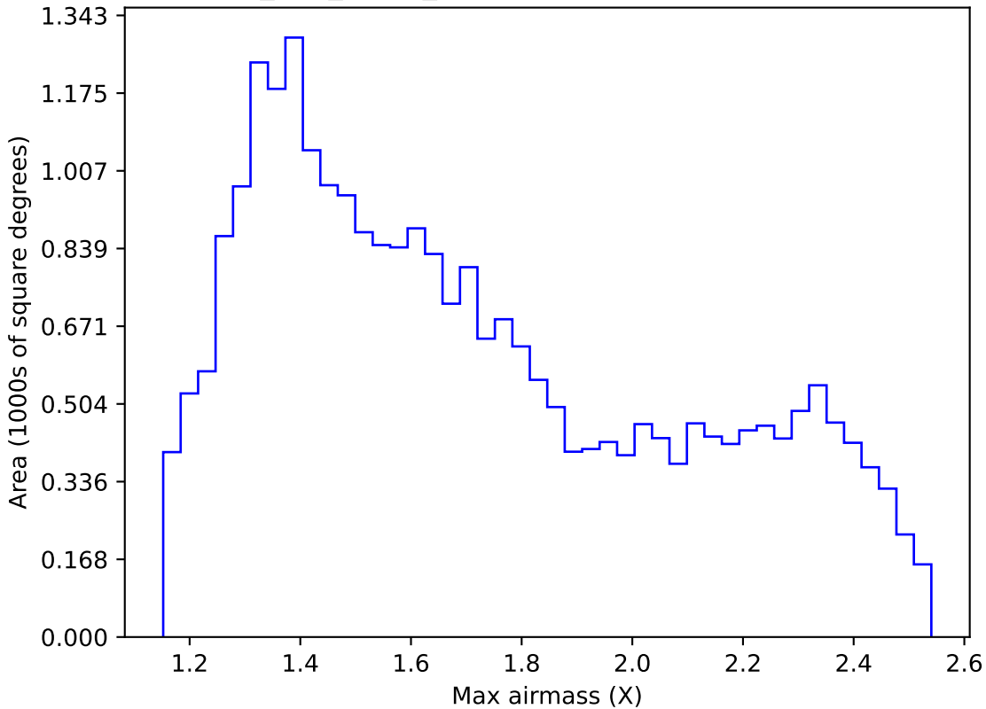
too_100_1v3.4_10yrs Yr 1 r band: Max airmass
