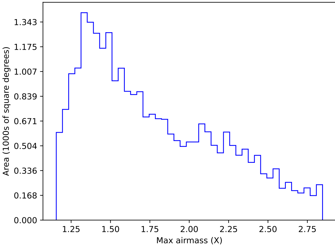
too_100_1v3.4_10yrs Yr 1 i band: Max airmass
