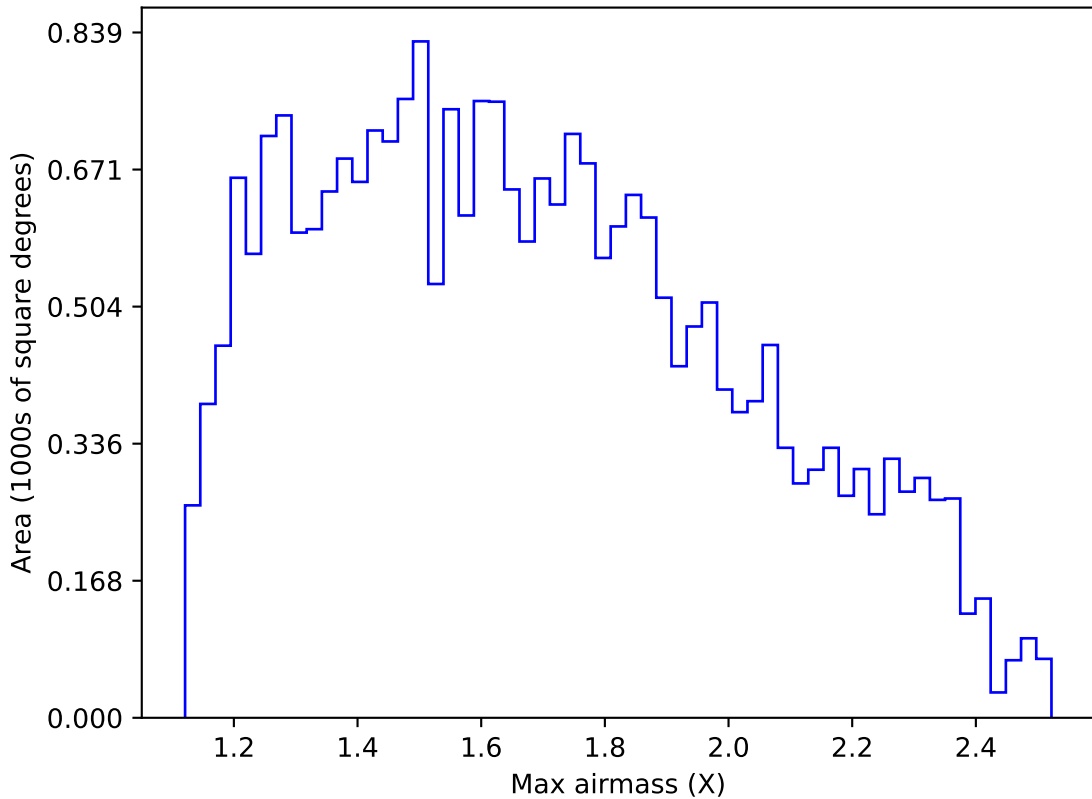
too_100_1v3.4_10yrs Yr 1 g band: Max airmass
