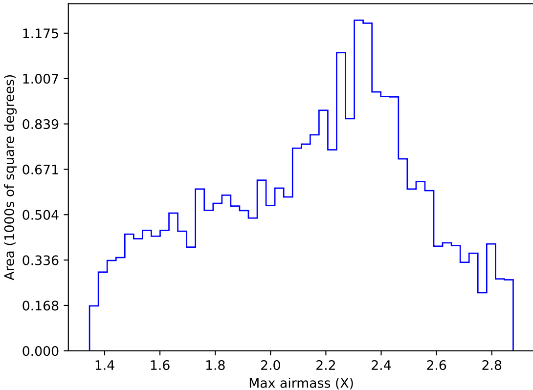
too_100_1v3.4_10yrs Yr 1 all bands: Max airmass
