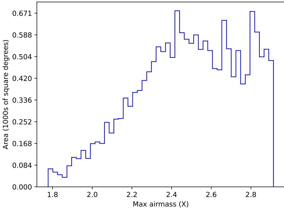
too_100_1v3.4_10yrs WFD z band: Max airmass
