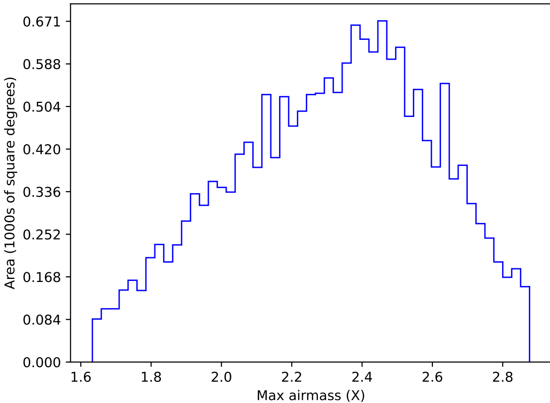
too_100_1v3.4_10yrs WFD y band: Max airmass
