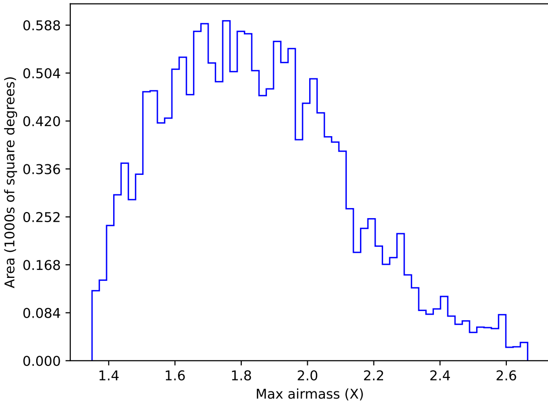
too_100_1v3.4_10yrs WFD u band: Max airmass
