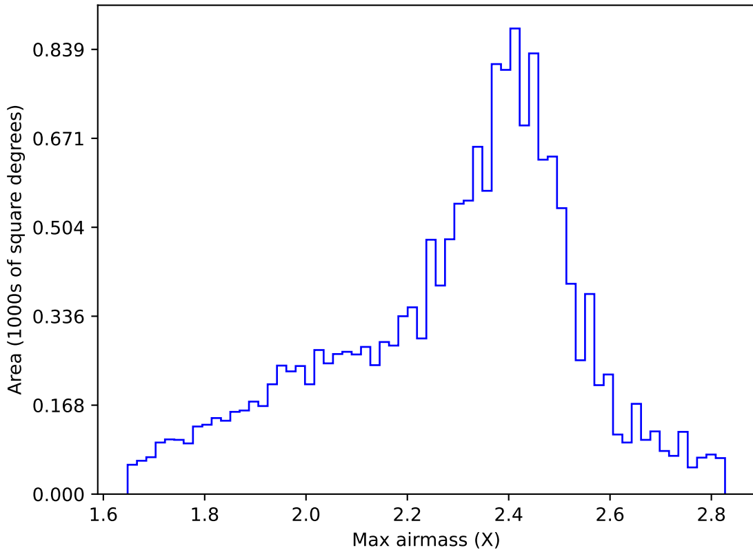
too_100_1v3.4_10yrs WFD r band: Max airmass
