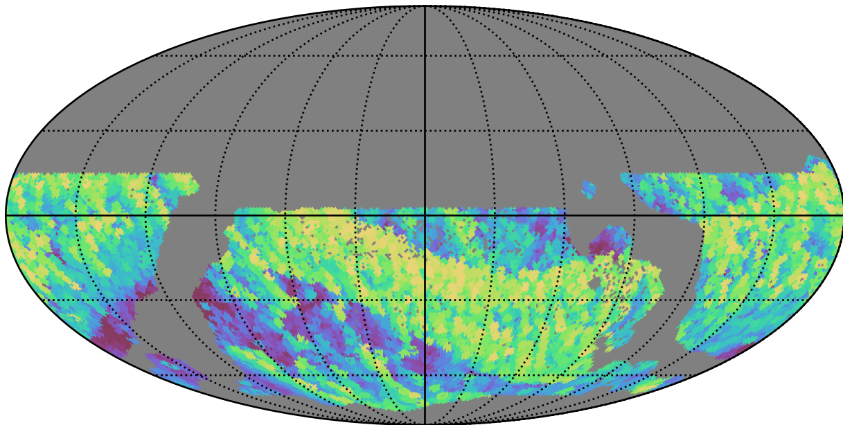
too_100_1v3.4_10yrs WFD i band: Max airmass
