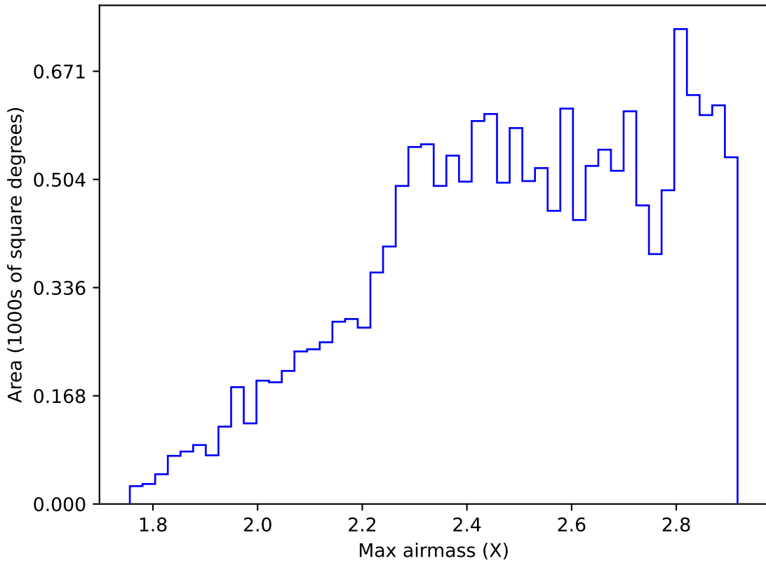
too_100_1v3.4_10yrs WFD i band: Max airmass
