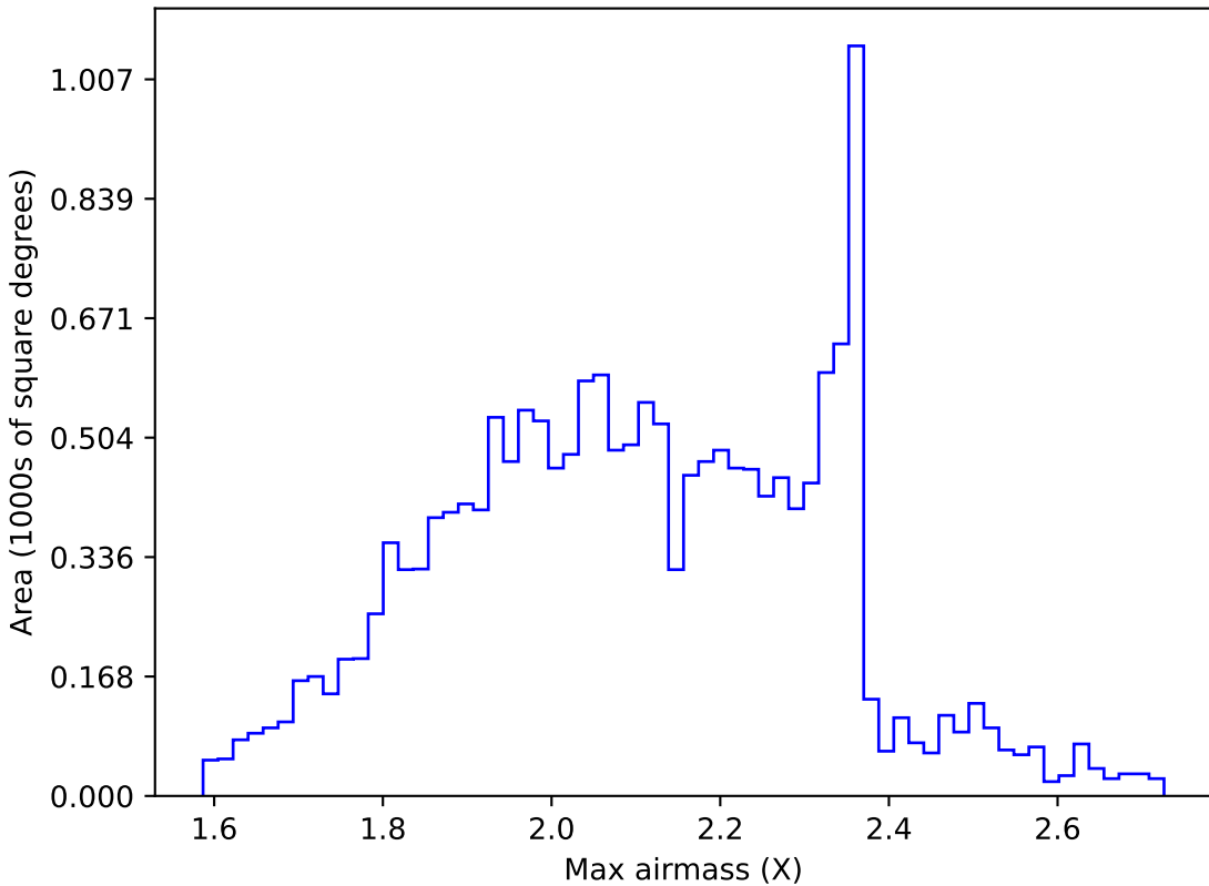
too_100_1v3.4_10yrs WFD g band: Max airmass
