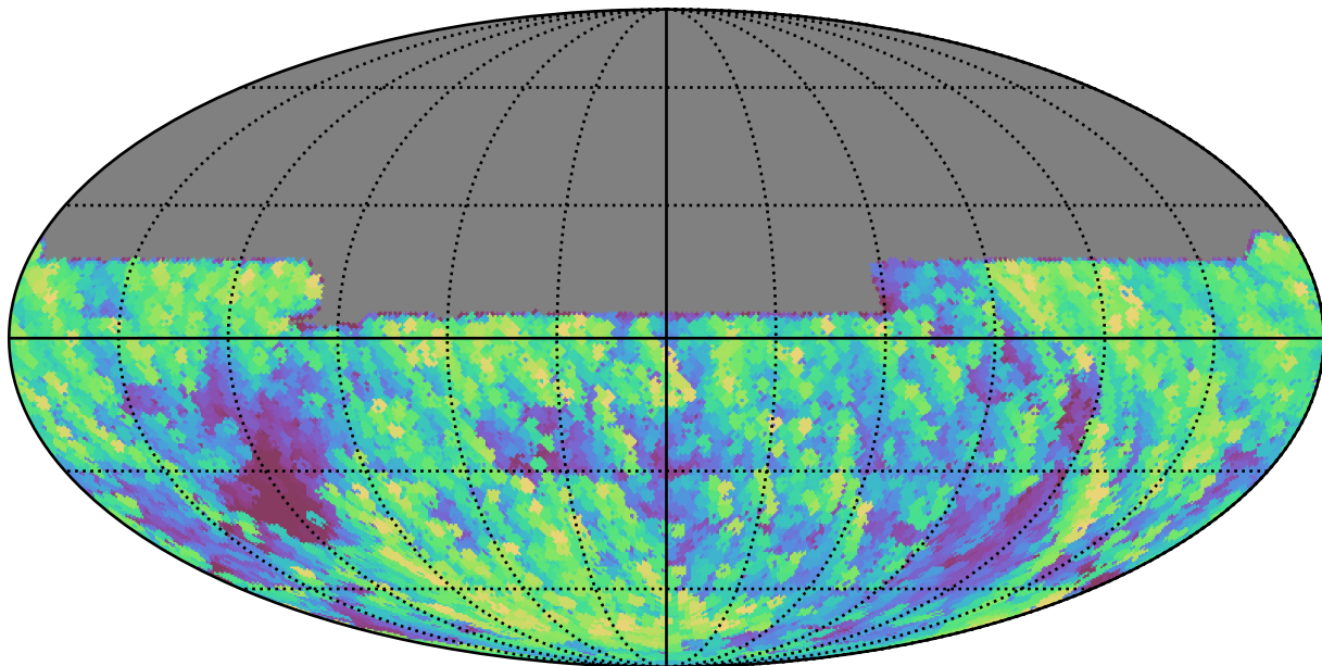
too_100_1v3.4_10yrs All sky y band: Max airmass
