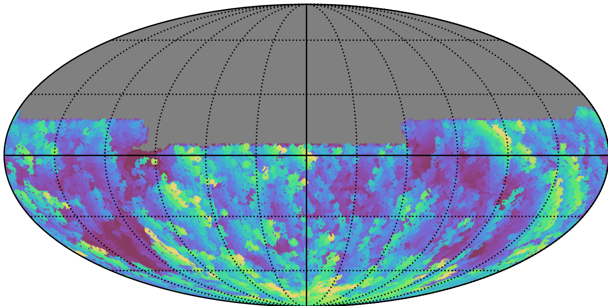
too_100_1v3.4_10yrs All sky u band: Max airmass
