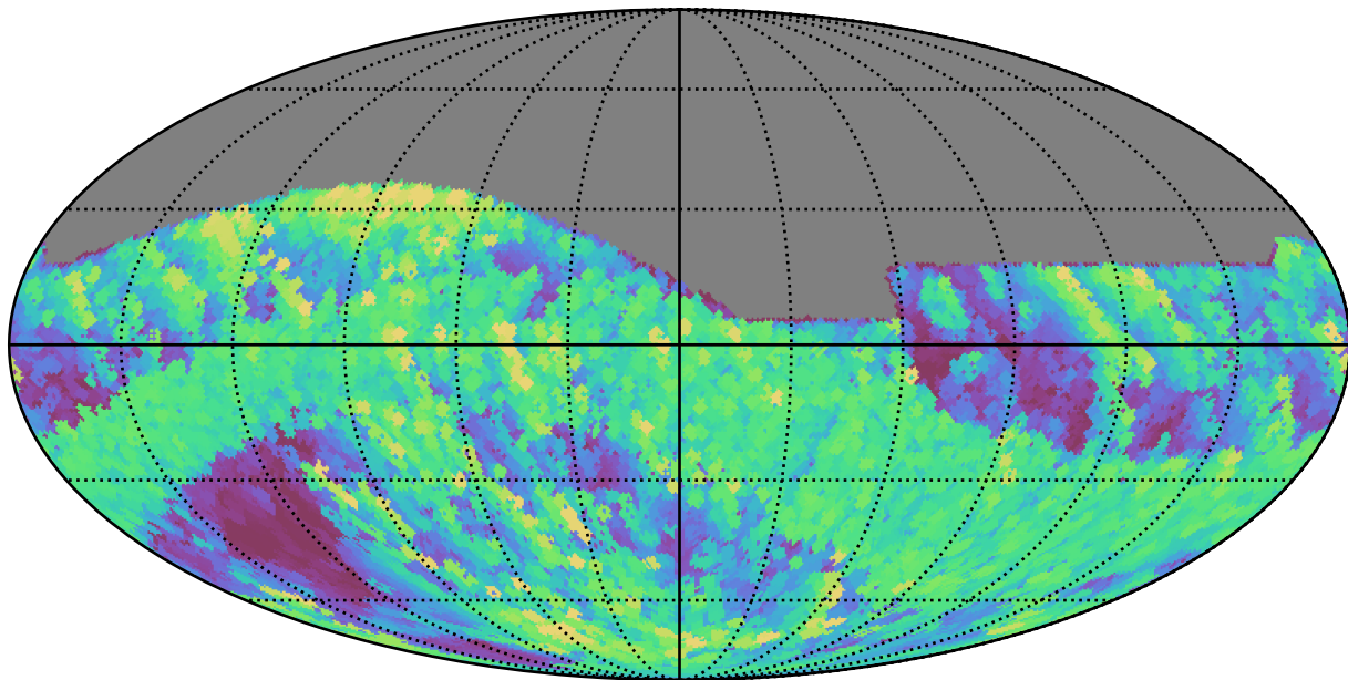
too_100_1v3.4_10yrs All sky r band: Max airmass
