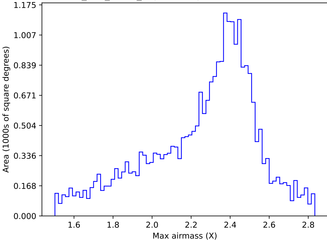
too_100_1v3.4_10yrs All sky r band: Max airmass
