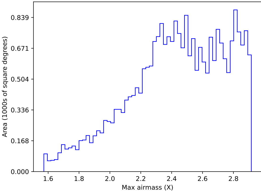
too_100_1v3.4_10yrs All sky i band: Max airmass
