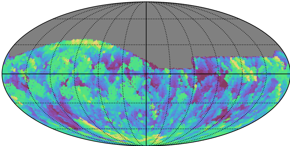
too_100_1v3.4_10yrs All sky g band: Max airmass
