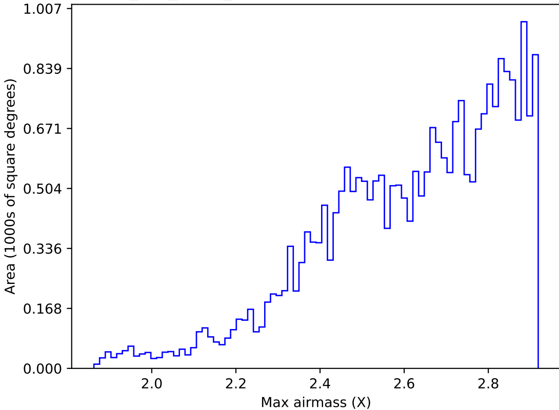
too_100_1v3.4_10yrs All sky all bands: Max airmass
