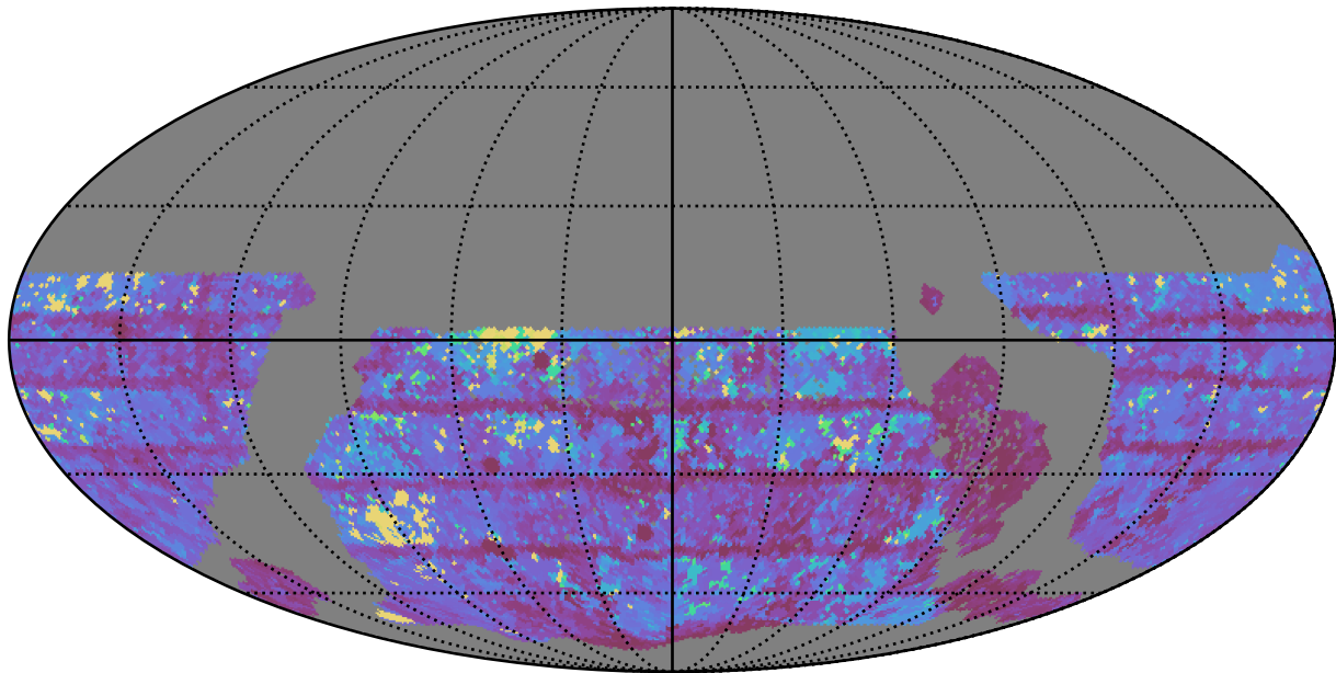
too_100_1v3.4_10yrs WFD z band: Max Inter-Night Gap
