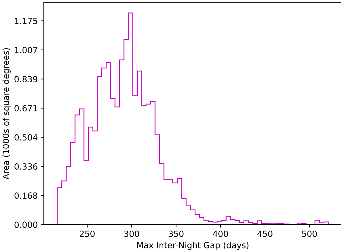
too_100_1v3.4_10yrs WFD z band: Max Inter-Night Gap
