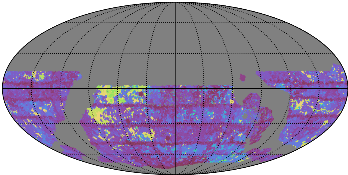
too_100_1v3.4_10yrs WFD y band: Max Inter-Night Gap
