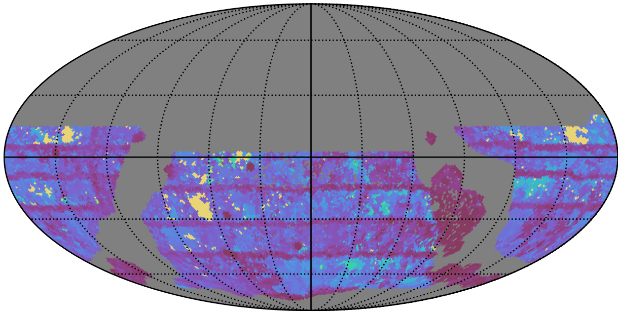
too_100_1v3.4_10yrs WFD r band: Max Inter-Night Gap
