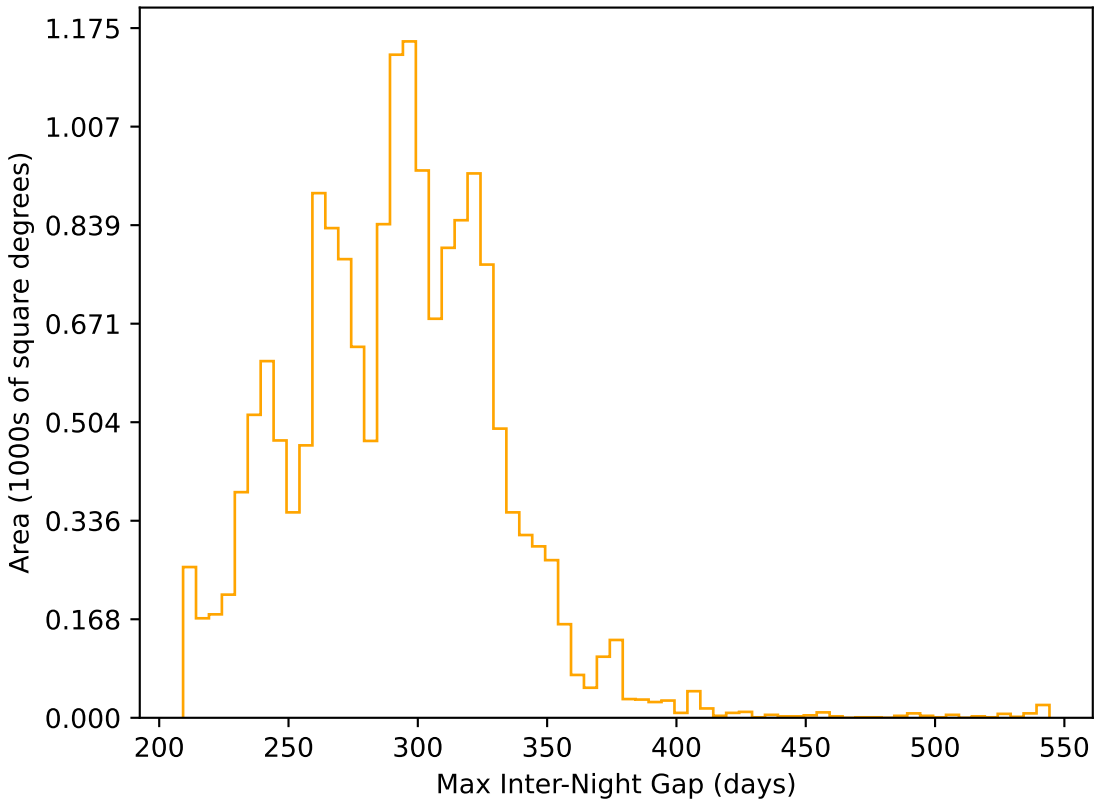
too_100_1v3.4_10yrs WFD r band: Max Inter-Night Gap
