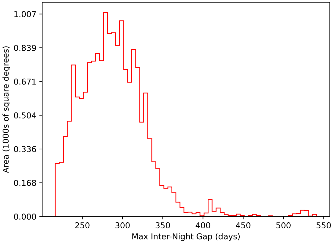
too_100_1v3.4_10yrs WFD i band: Max Inter-Night Gap
