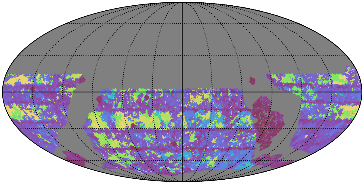
too_100_1v3.4_10yrs WFD g band: Max Inter-Night Gap
