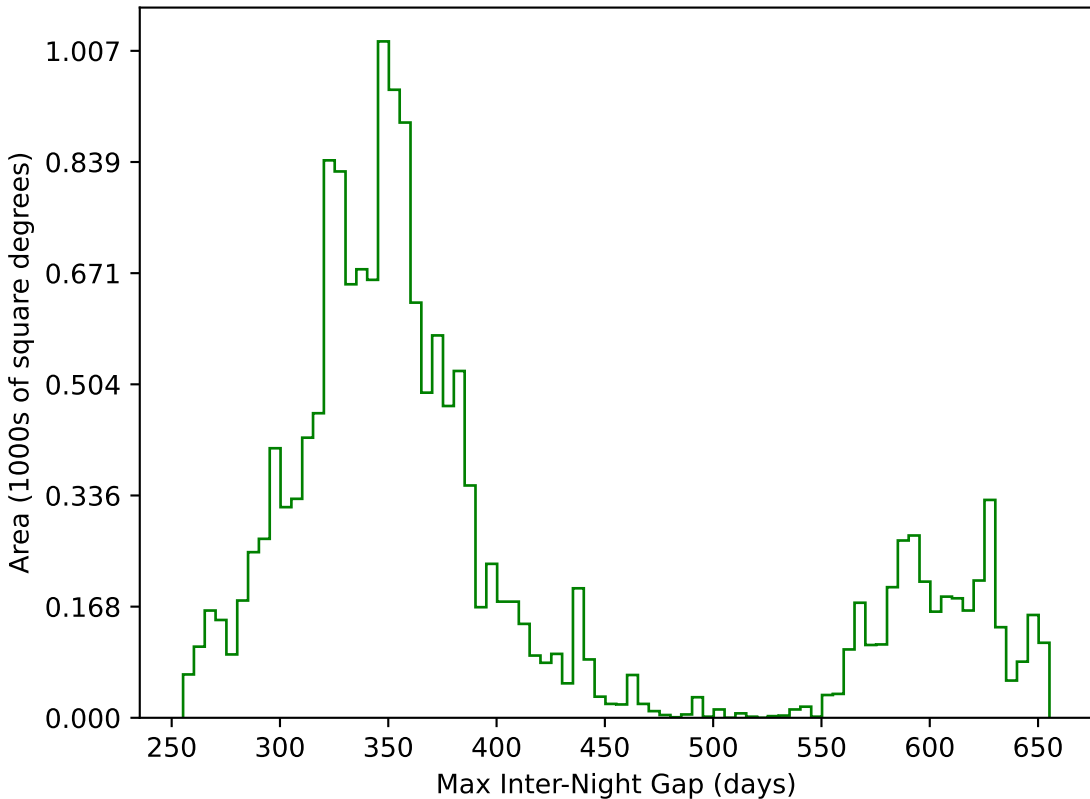
too_100_1v3.4_10yrs WFD g band: Max Inter-Night Gap
