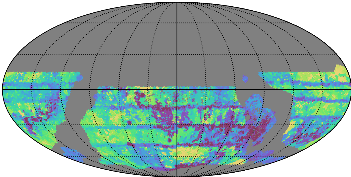
too_100_1v3.4_10yrs WFD all bands: Max Inter-Night Gap
