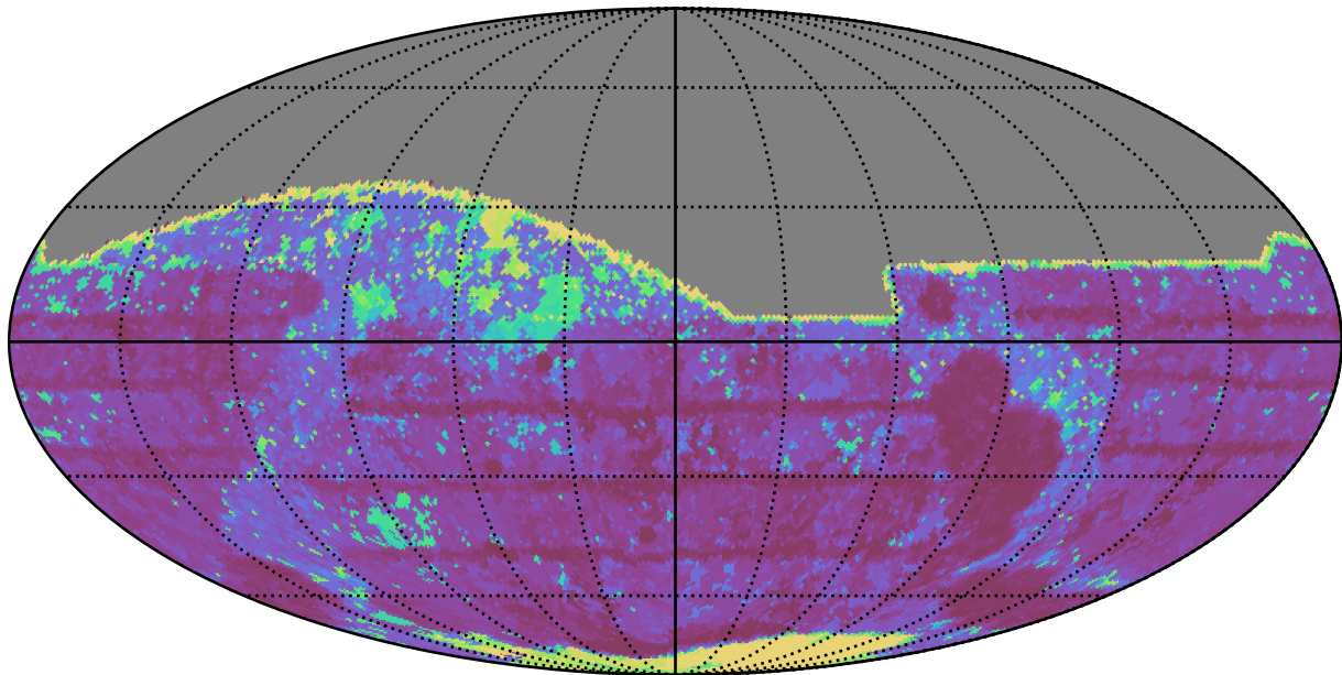
too_100_1v3.4_10yrs All sky z band: Max Inter-Night Gap
