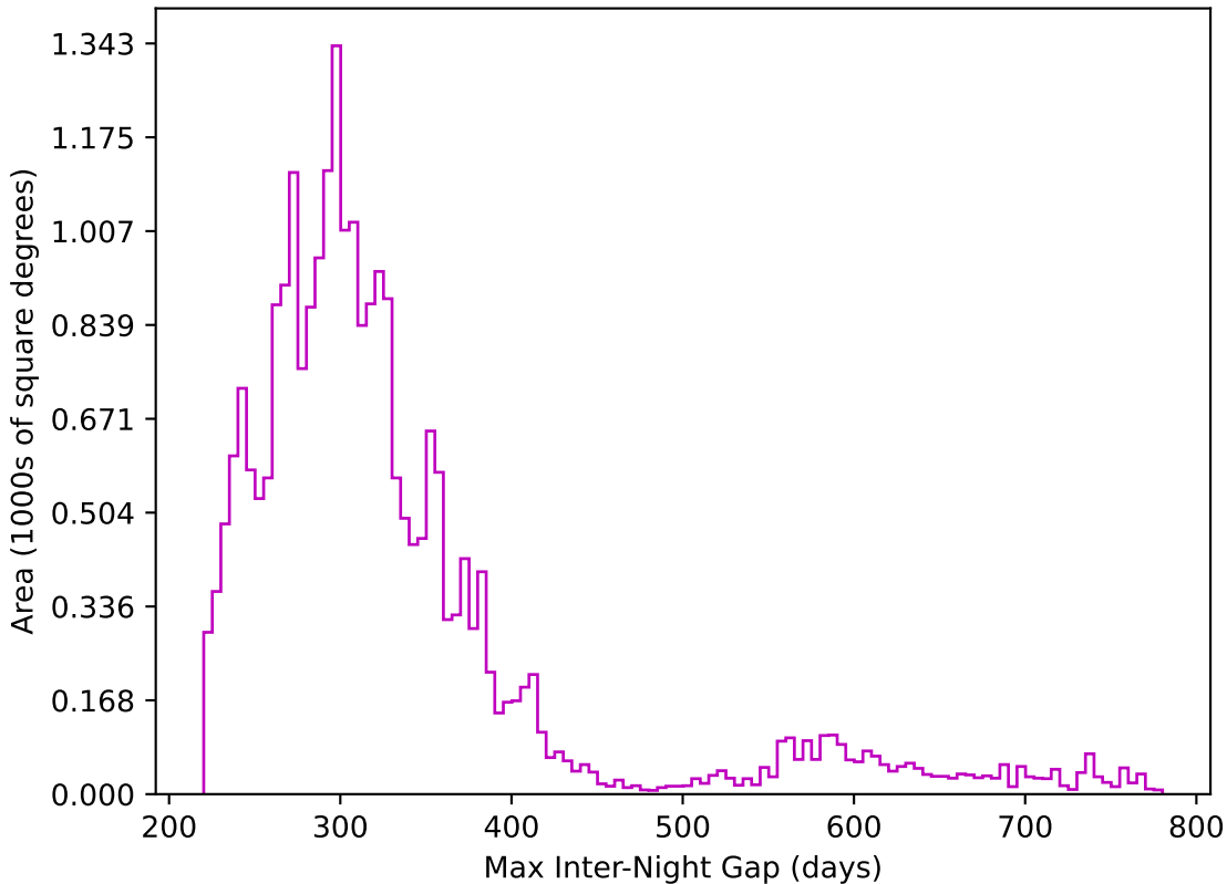
too_100_1v3.4_10yrs All sky z band: Max Inter-Night Gap
