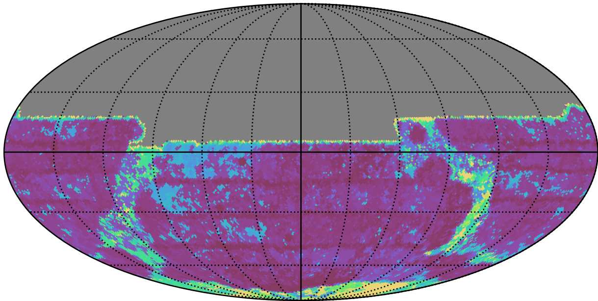
too_100_1v3.4_10yrs All sky y band: Max Inter-Night Gap
